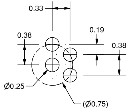
HOLE PATTERN DETAIL Ø0.25 HOLES ON 0.38 STAGGERED CENTERS
