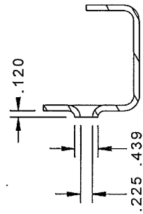
Section View of Punch Pattern
