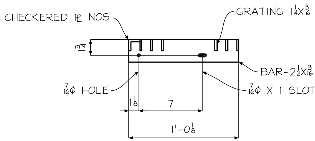
6 - TREADS - 4TI
