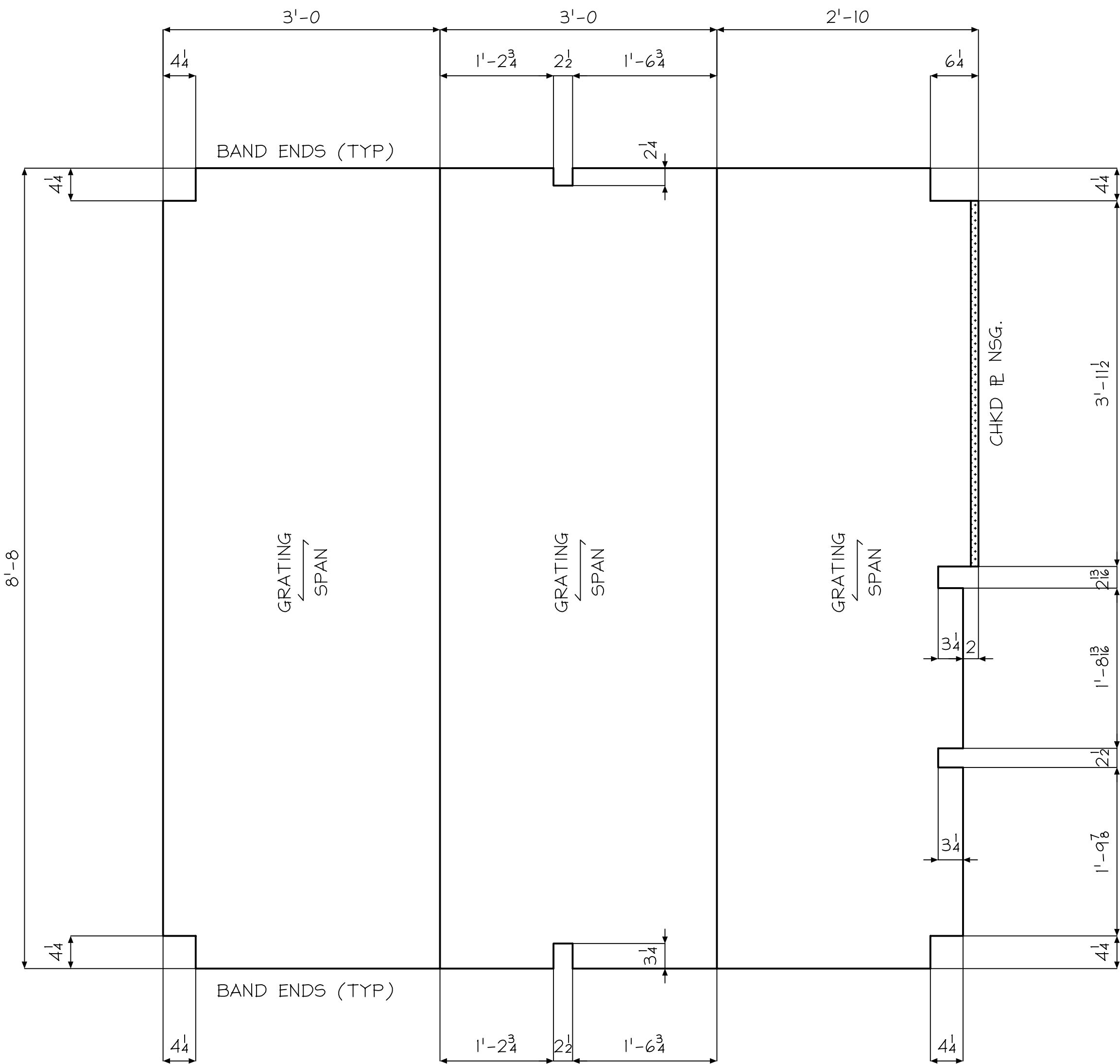
1 - GRTG - 4M2
