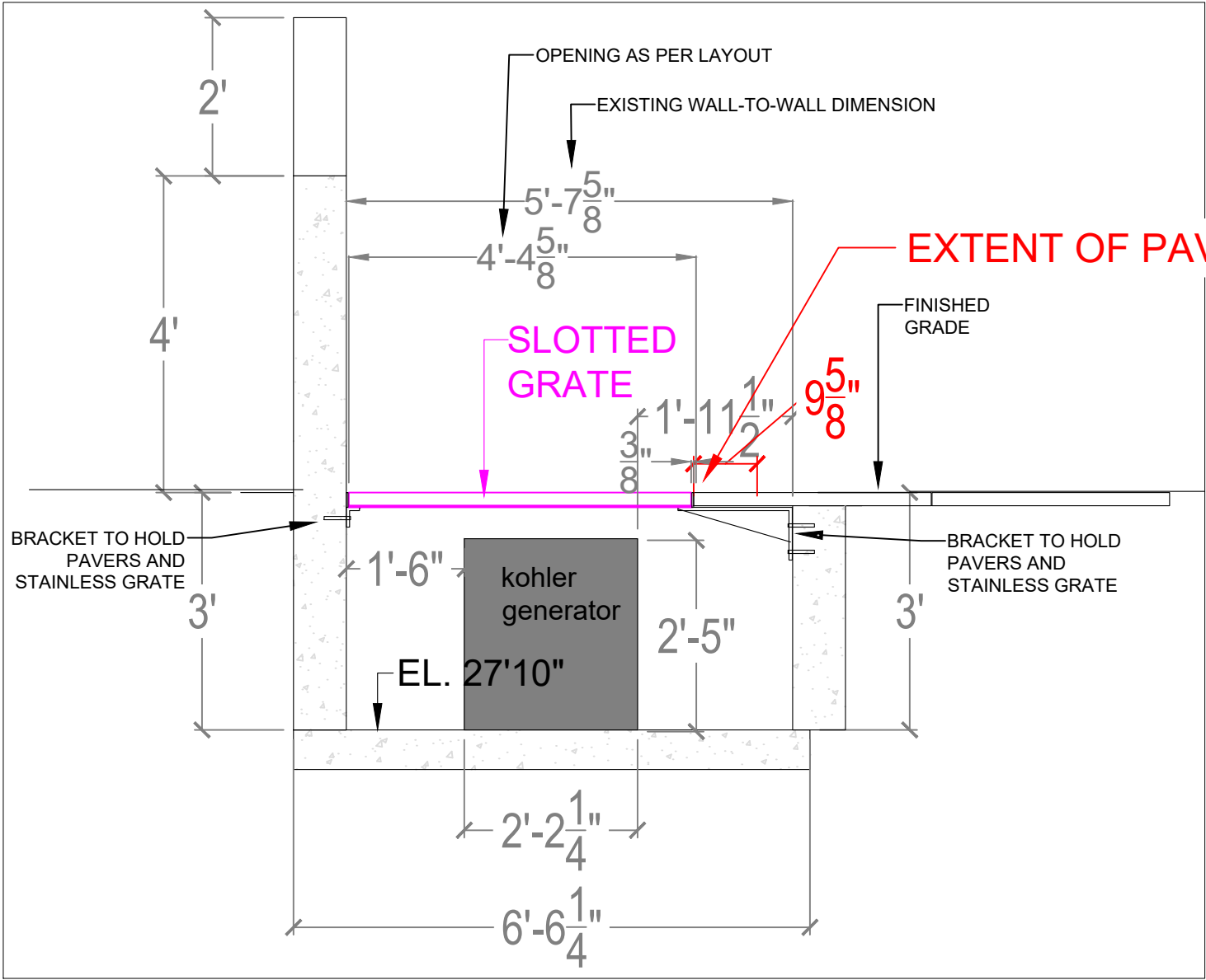
GENERATOR ENCLOSURE SECTION VIEW
