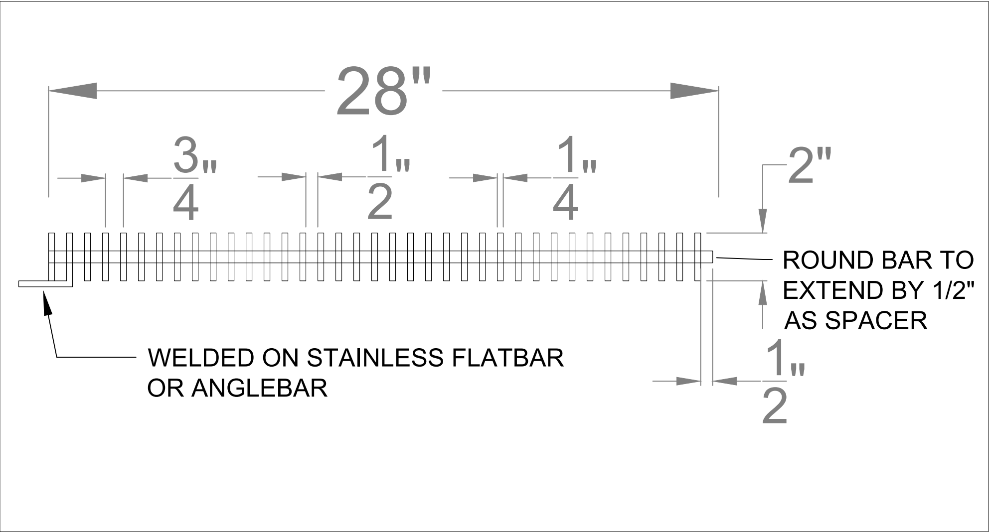
GENERATOR PLAN VIEW. SCALE 3" = 1'-0"
