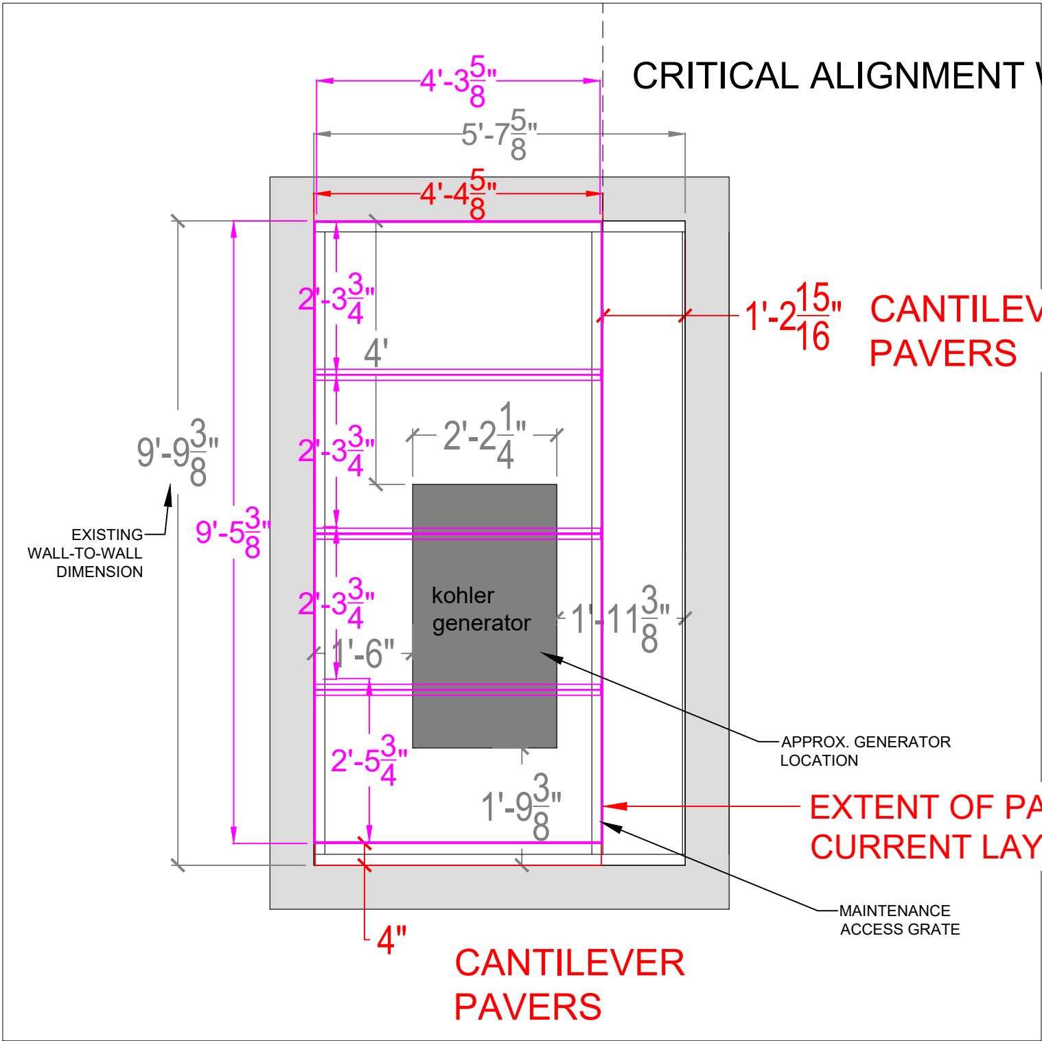
GENERATOR ENCLOSURE PLAN VIEW
