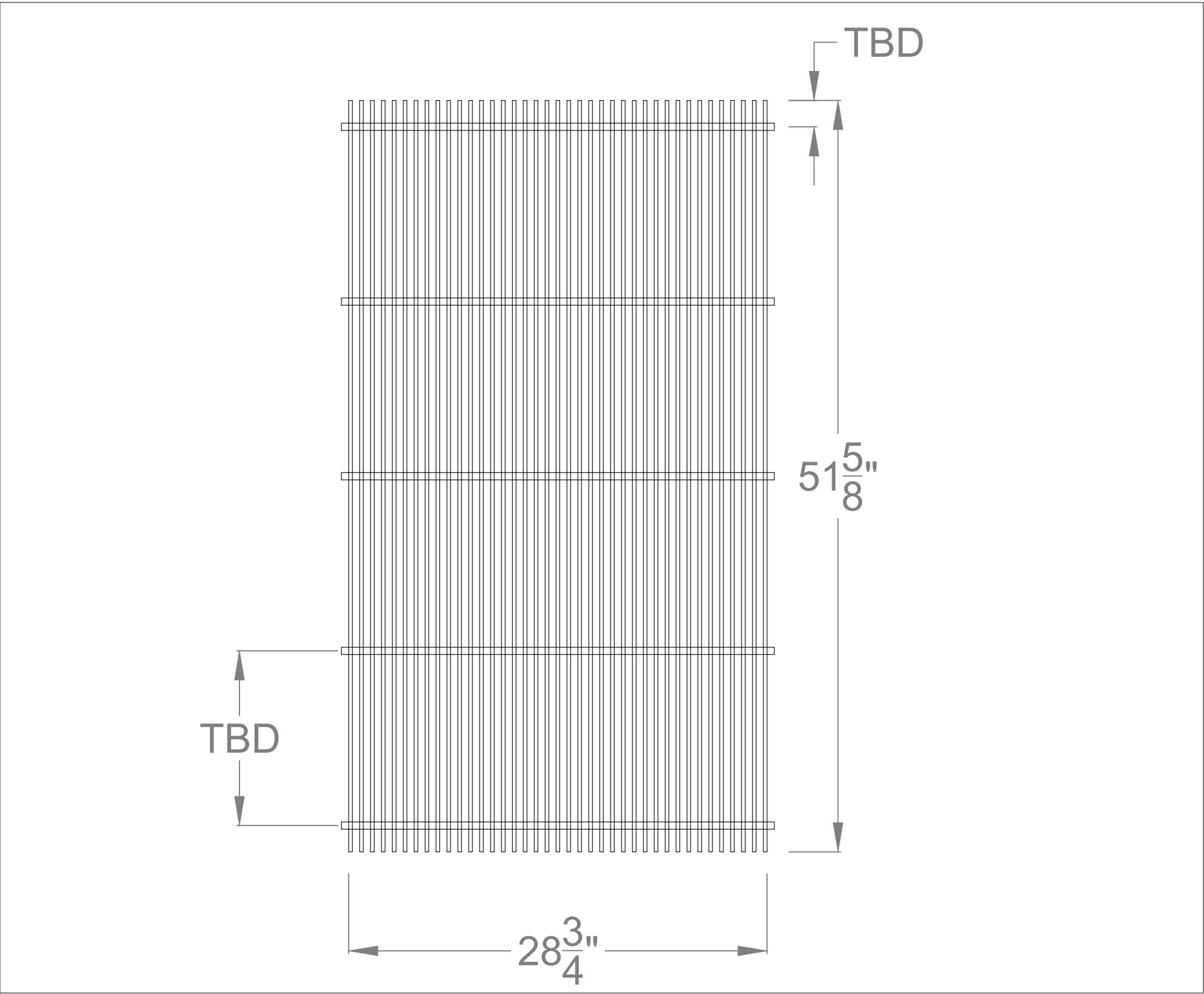
GRATE PLAN VIEW. SCALE 1&1/2" = 1'-0"
