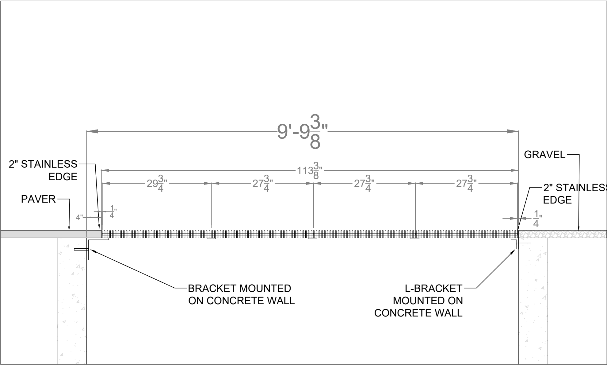
GENERATOR SECTION VIEW
