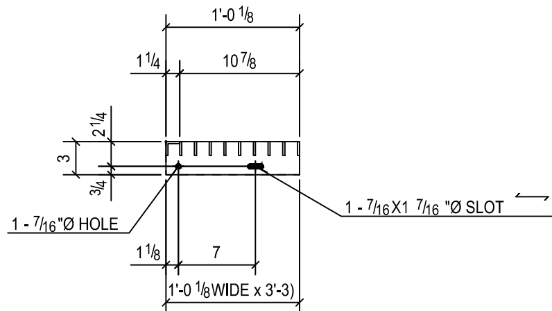
12 - TREADS - 34M1
