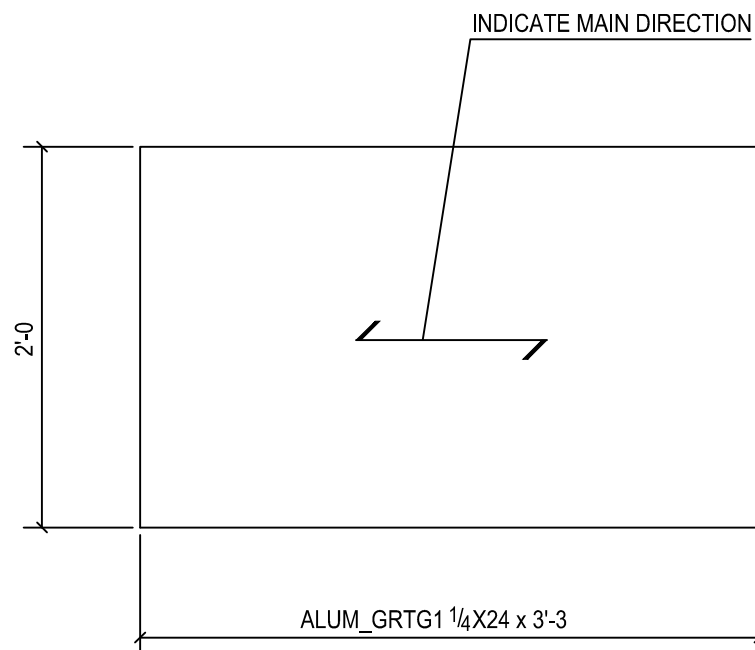
2 - GRATINGS - 34GRT1
