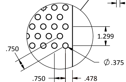
DETAIL A SCALE 1 : 4
