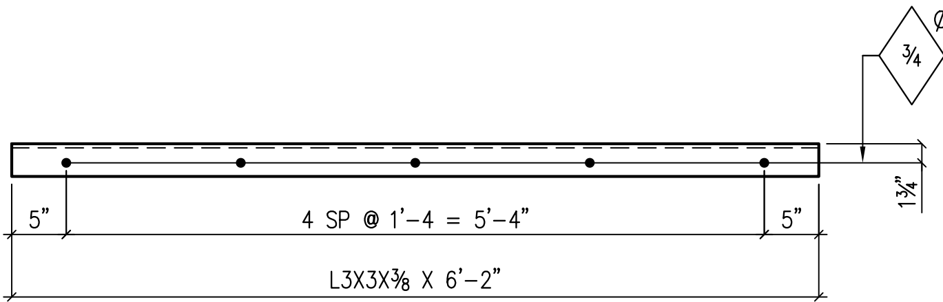
2 ANGLES THUS MK 28A2
