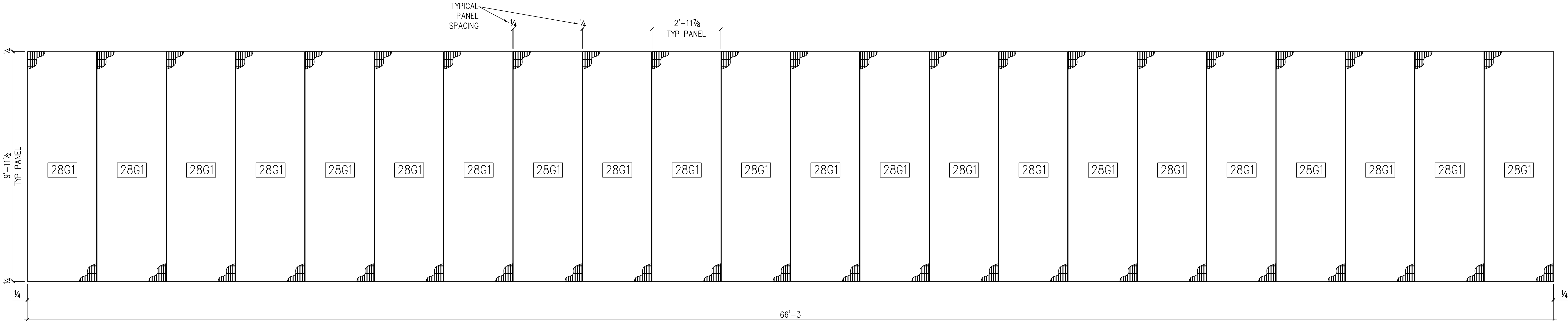
ONE AREA OF GRATING THUS A. N. MK 28G1
