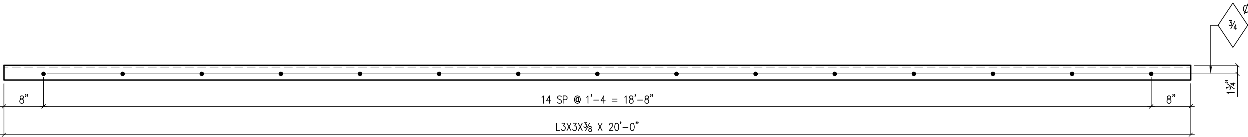
6 ANGLES THUS MK 28A1
