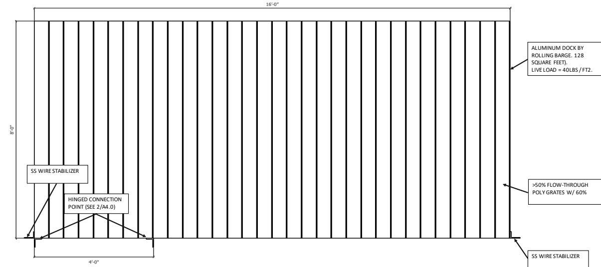
2 DOCK PLAN NTS
