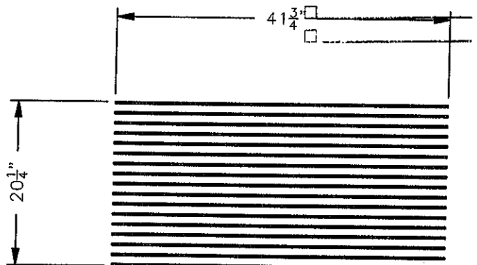
DECK D MATERIAL: 1/4" X 1" ON 1" CENTERS OPEN 21 x 42"
