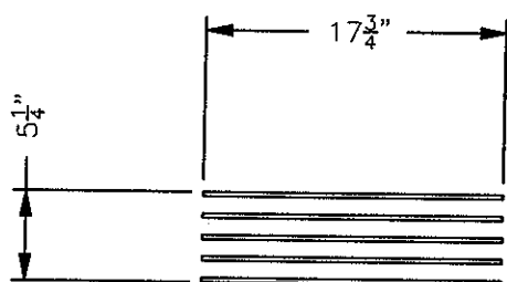
DECK E MATERIAL: 1/4" X 1" ON 1" CENTERS
