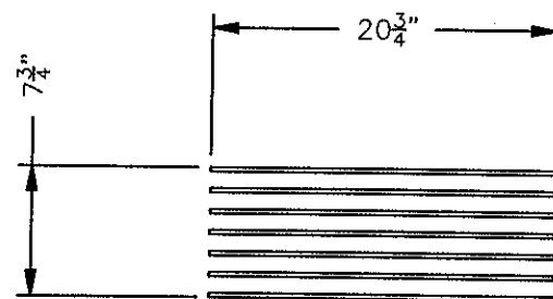
DECK F MATERIAL: 1/4" X 1" ON 1" CENTERS OPEN 9" x 21" 2 REQ'D
