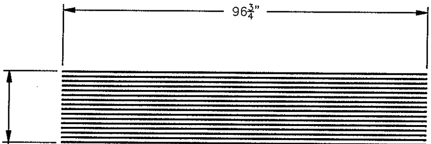
DECK C MATERIAL: 1/4" X 1" ON 1" CENTERS OPEN 20" x 97"
