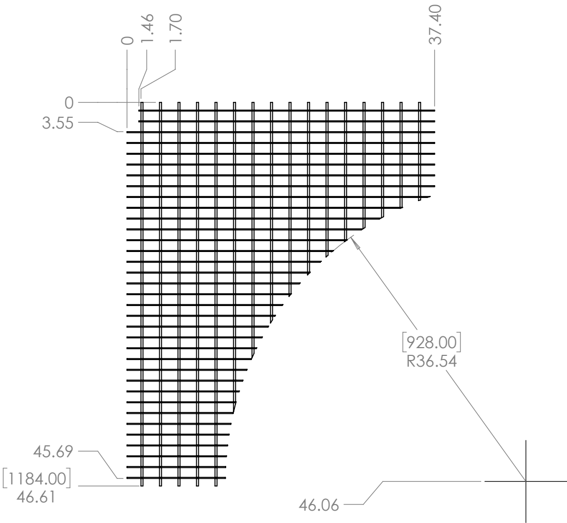
PN# 3878953 MULTI PIECE CONSTRUCTION
