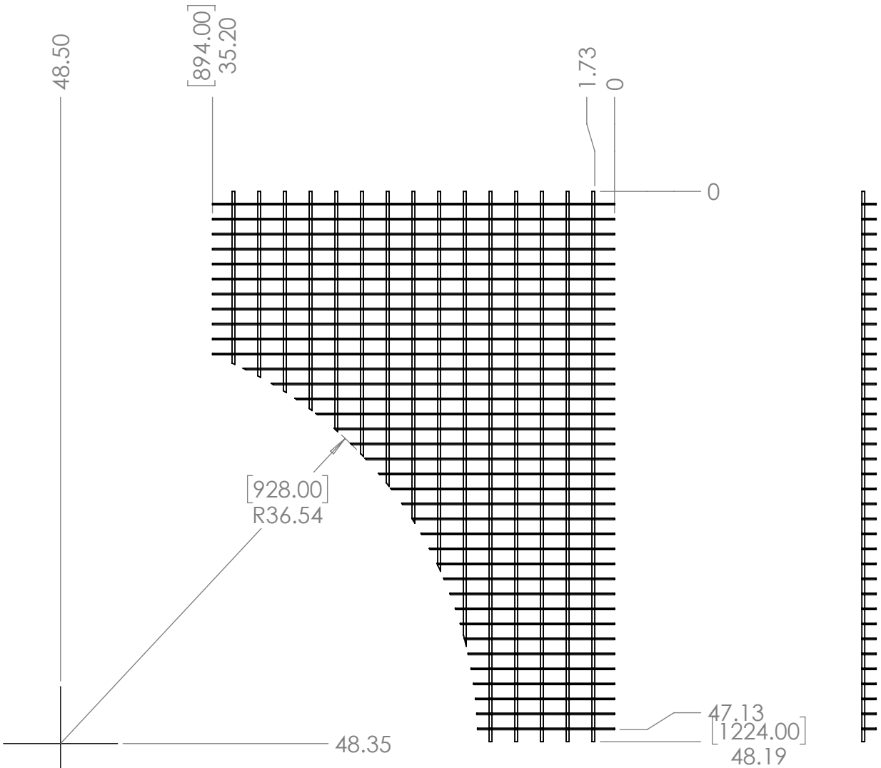
PN# 3878908 MULTI PIECE CONSTRUCTION
