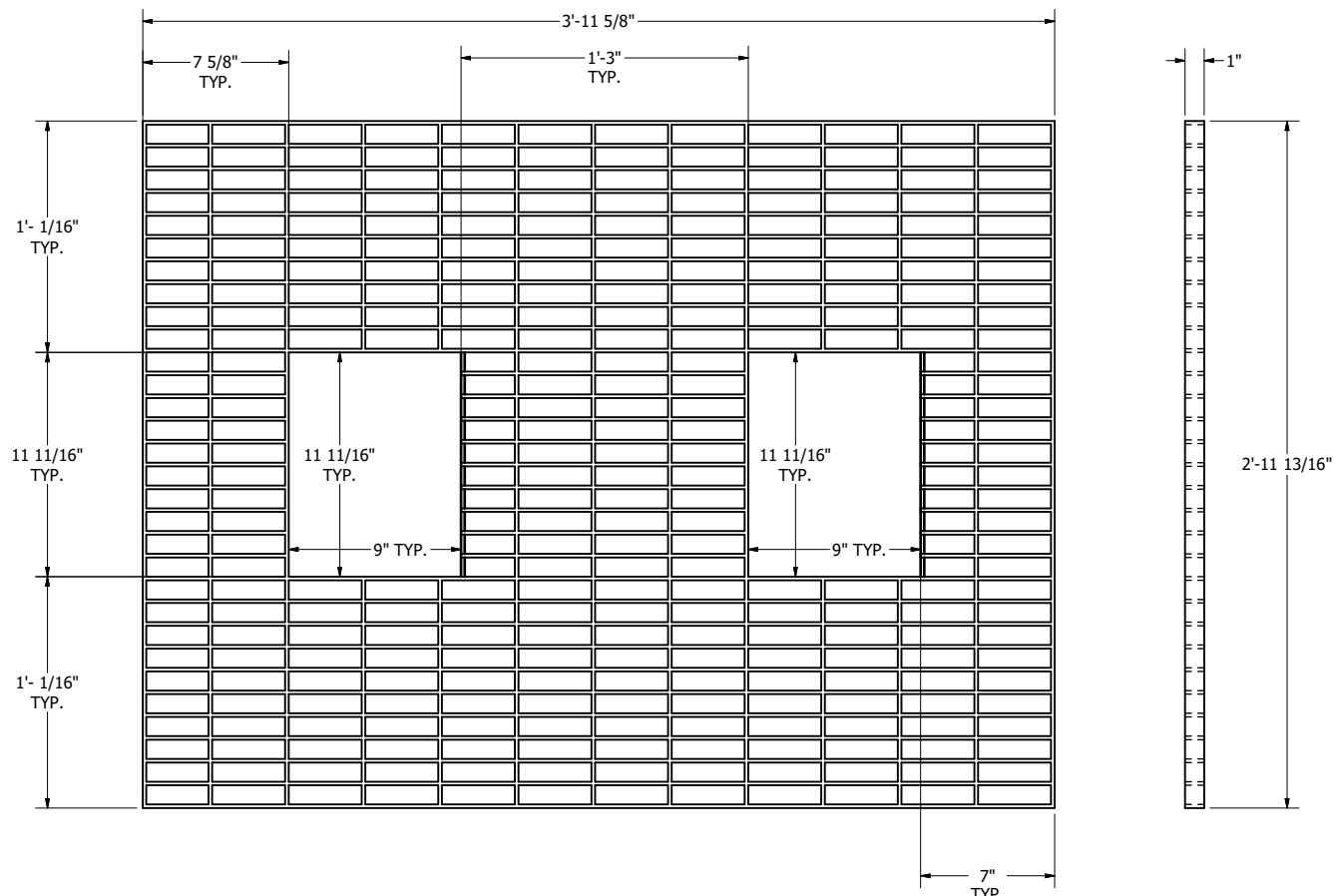
GRATING 2 CUTOUT FOR INNER FENCE POSTS ITEM #21
