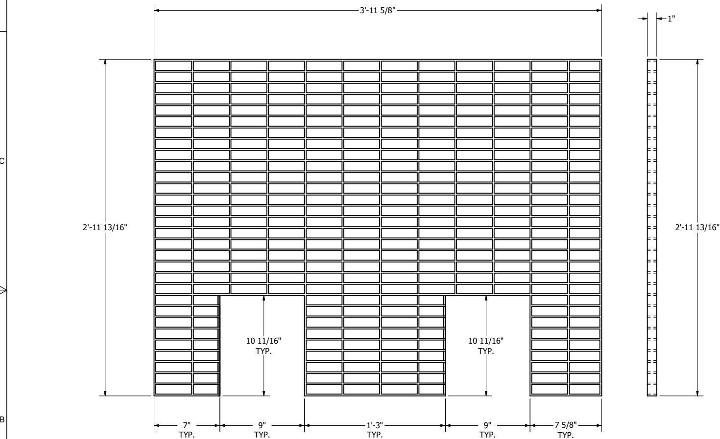
GRATING 1 CUTOUT FOR OUTER FENCE POSTS ITEM #20
