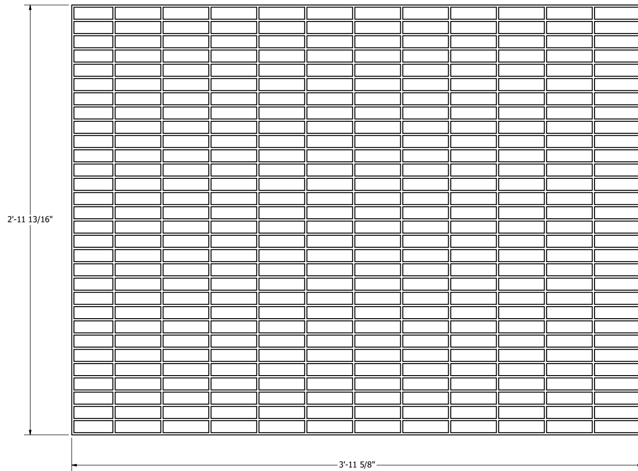
GRATING 5 TYP. ITEM #24
