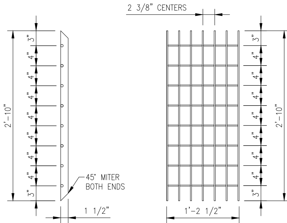
38W4-1 1/2"x1/4" - (1) GRATING PIECE 1'-2 1/2" X 2'-10"
