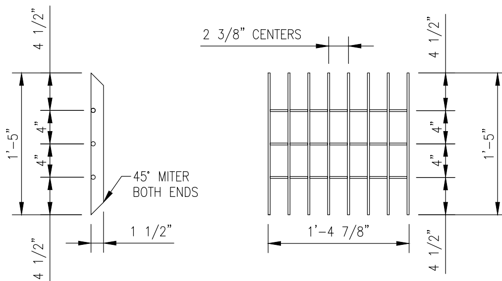
38W4-1 1/2"x1/4" - (2) GRATING PIECES 1'-4 7/8"x1'-5"
