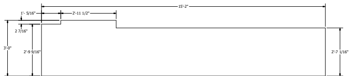
GRATING 4 SCALE 1 / 15
