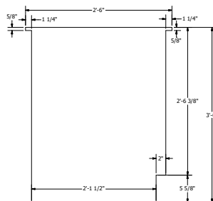
GRATING 11 SCALE 1 / 7
