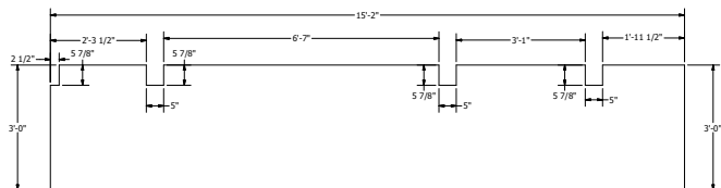
GRATING 9 SCALE 1 / 15
