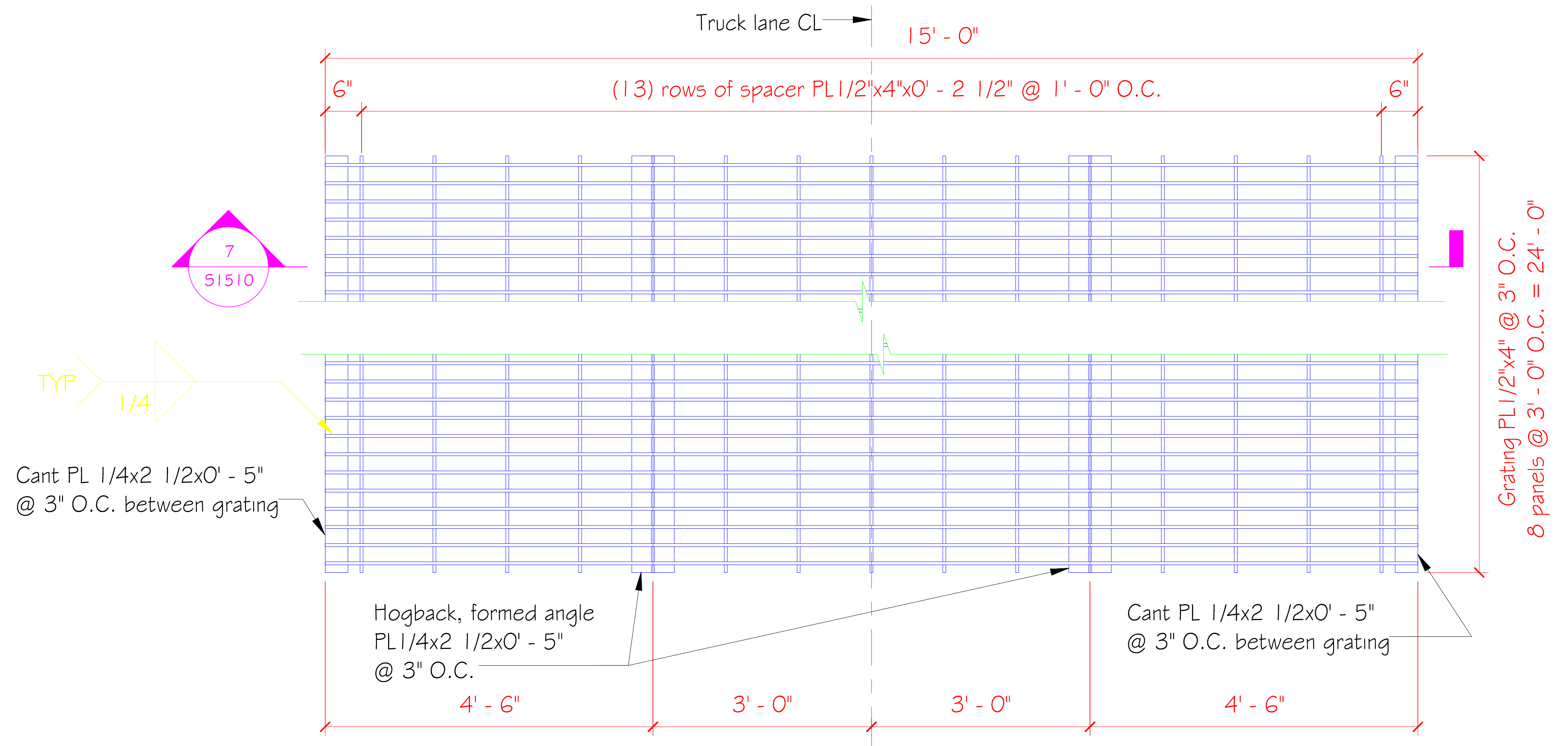
6 Detail- Truck RCV Grating 1/2" = 1'-0"
