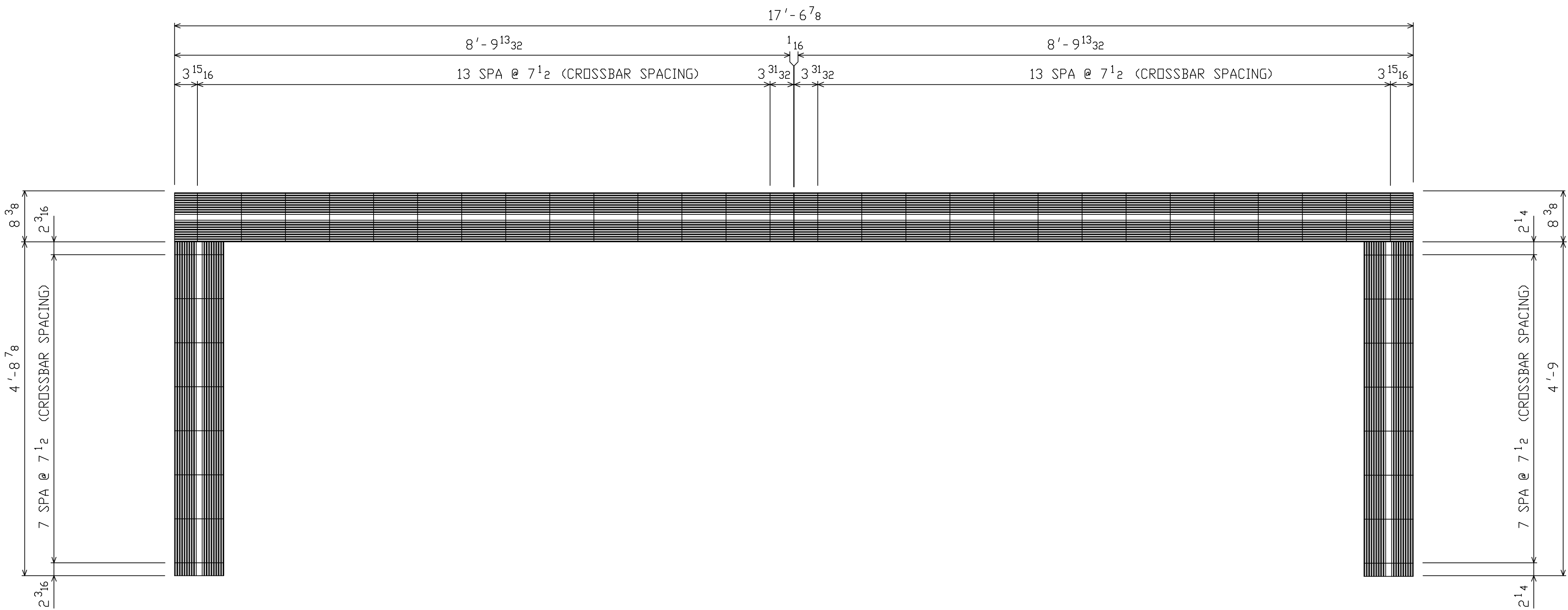
EAST/MIDDLE TRENCH GRATING PLAN
