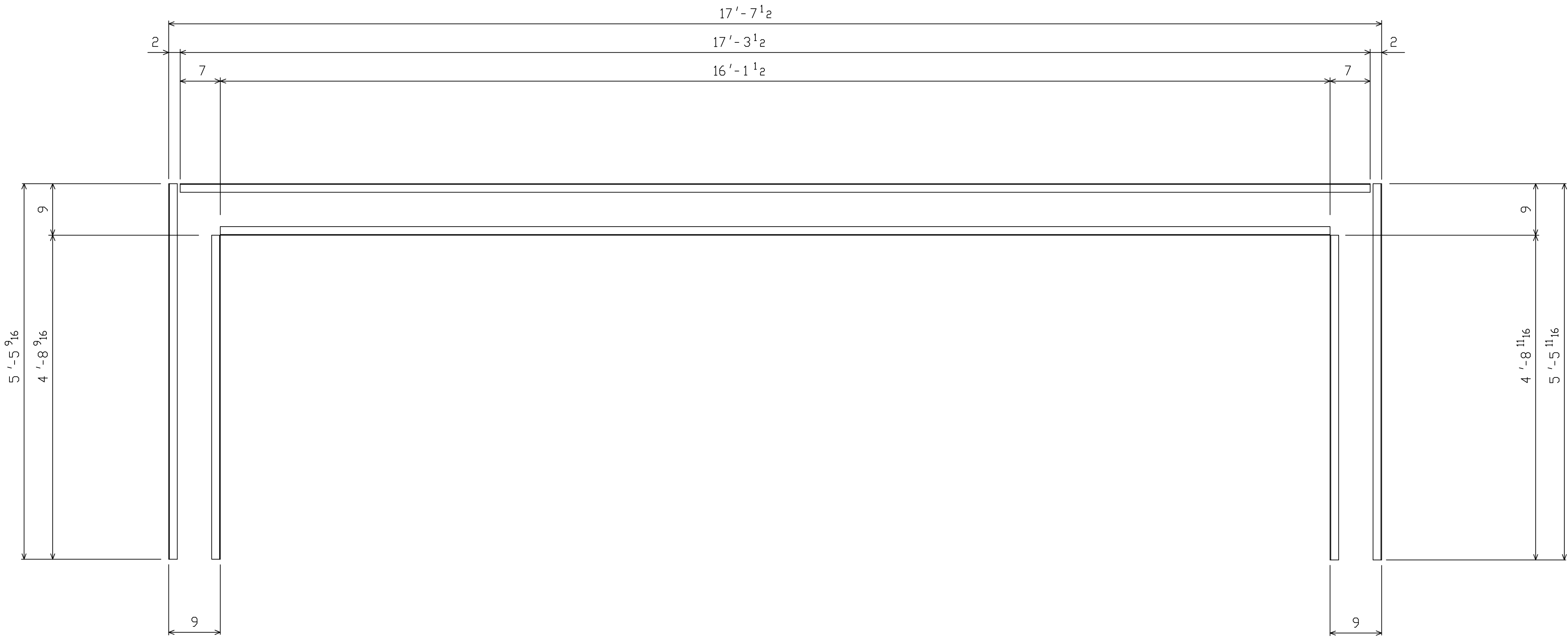
EAST/MIDDLE TRENCH ANGLE PLAN
