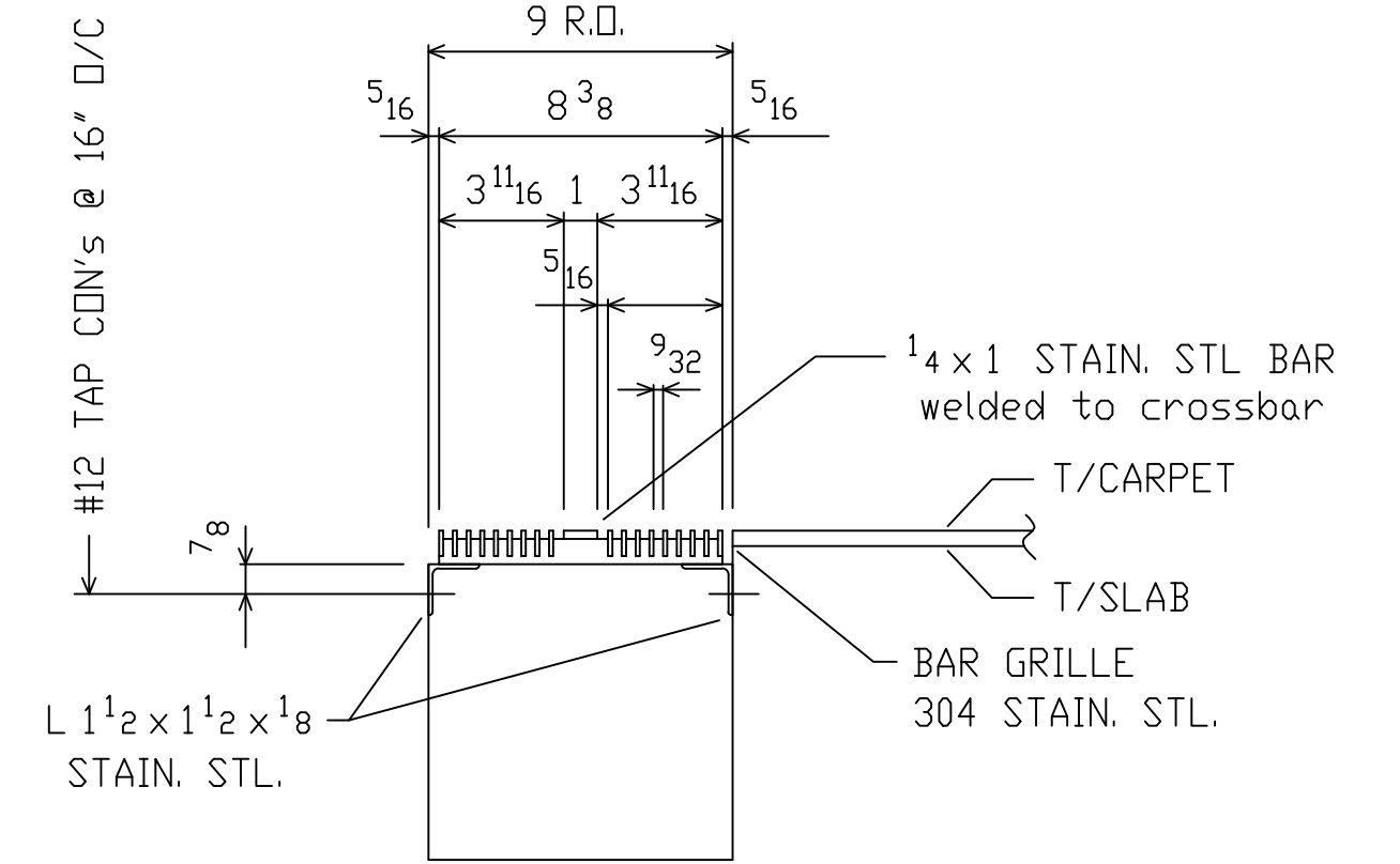
TYP CROSS SECTION THROUGH TRENCH
