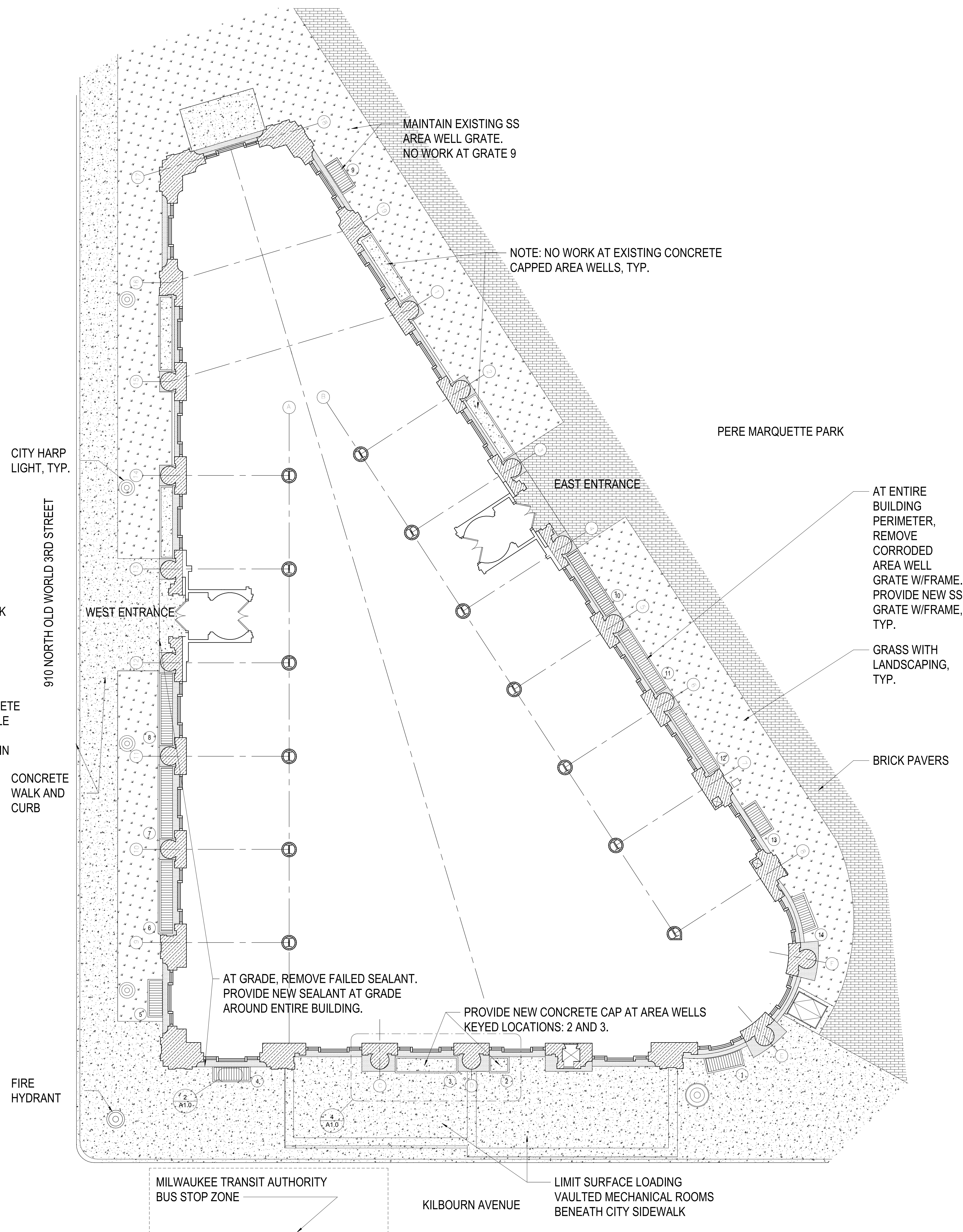
① LOCATIONS OF WINDOW AREA WELLS AT GRADE 1/8" = 1'-0"
