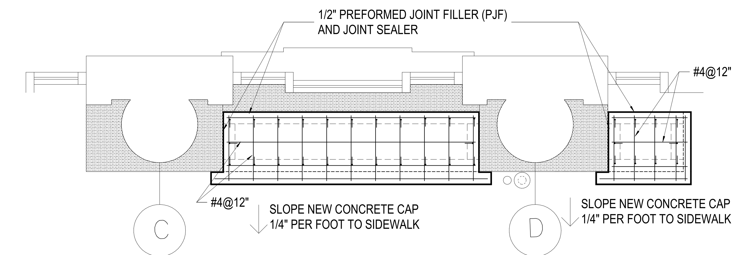
4 AREA WELL GRATE PLAN DETAILS 1/2" = 1'-0"
