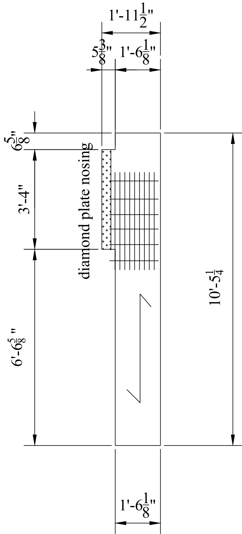
One Req'd -1 1/4 x 1/8"grating - mk "G8" 1 3/16" c/c bars (Galv)
