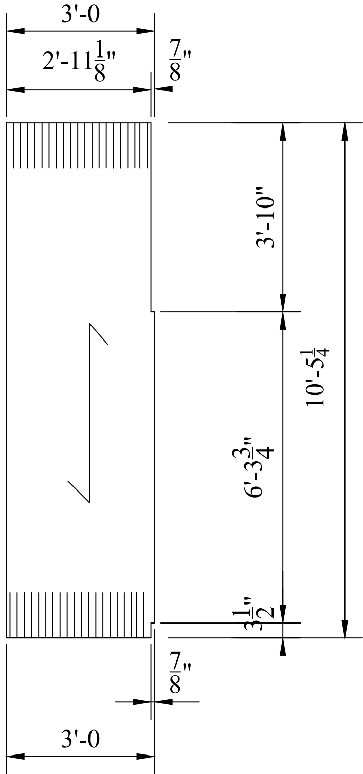
One Req'd -1 1/4 x 1/8"grating - mk "G7" 1 3/16" c/c bars (Galv)
