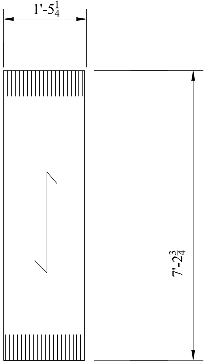
One Req'd -1 1/4 x 1/8"grating - mk "G7" 1 3/16" c/c bars (Galv)
