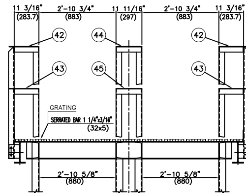
SECTION "A" (FOR "1~4, 6~10 F.L." ONLY)
