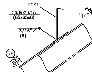
DETAIL "P"
