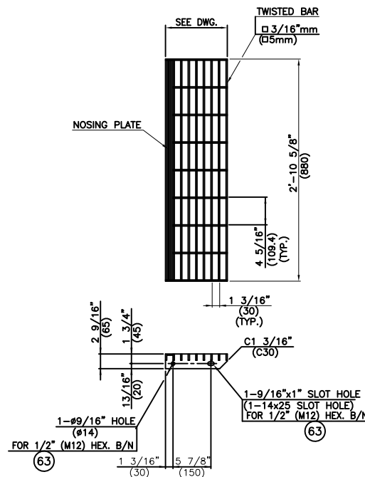
STAIR TREADS (F.B 1 1/4'x3/16" SERRATED) STAIR TREADS (32x5 SERRATED)
