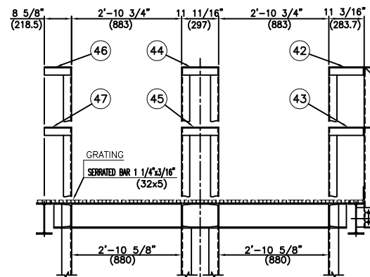
SECTION "B" (FOR "5 F.L." ONLY)
