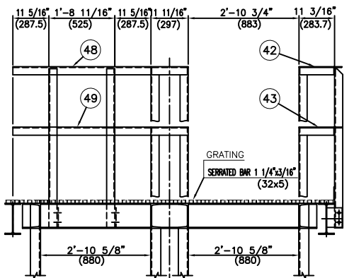
SECTION "C" (FOR "11 F.L." ONLY)
