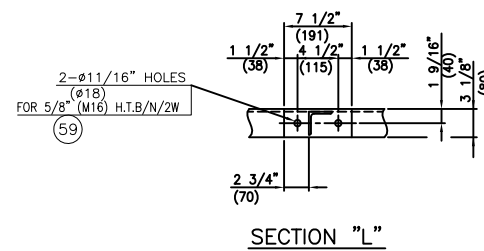
SECTION "L"
