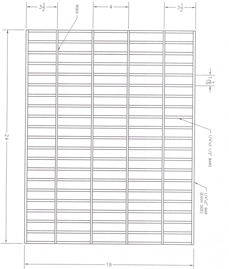
1 TOP VIEW
