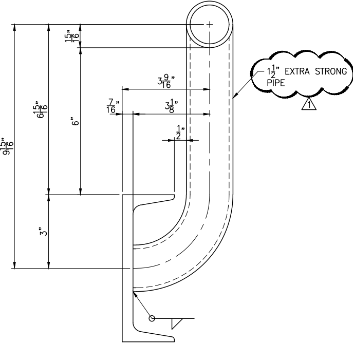
2 SECTION 6"=1'-0"
