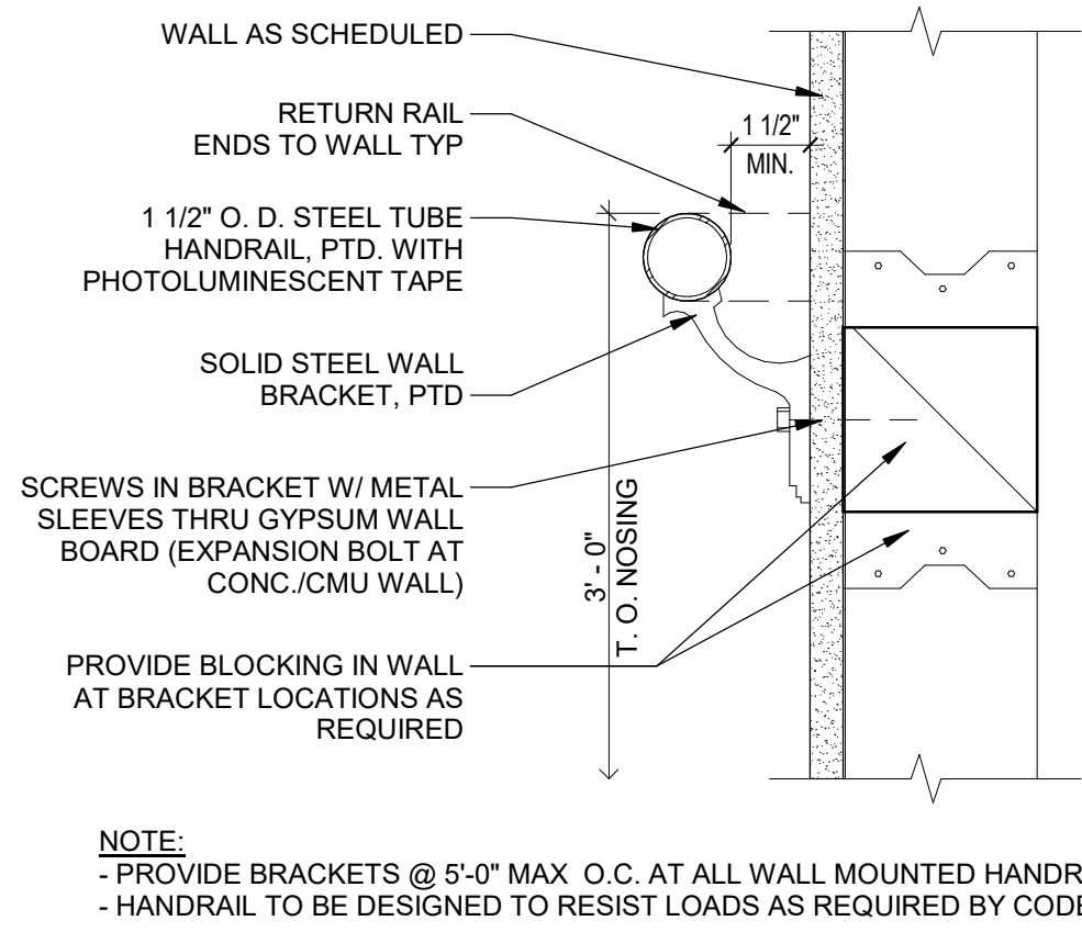
9 STAIR DETAIL - HANDRAIL - SECTION - WALL MOUNT - TYP 3" = 1'-0"
