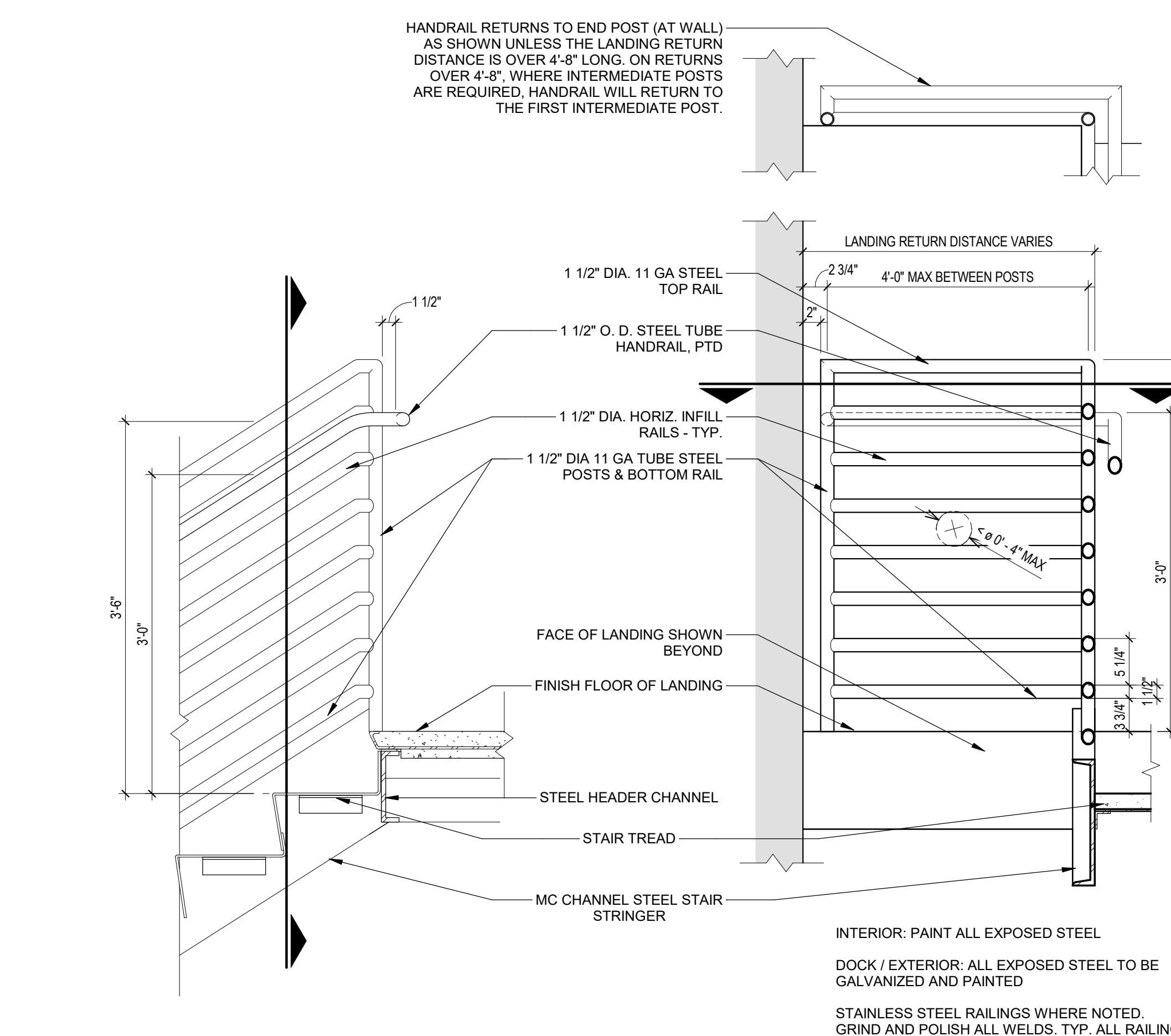
1 STAIR DETAIL - GUARDRAIL - HORIZONTAL INFILL 1" = 1'-0"
