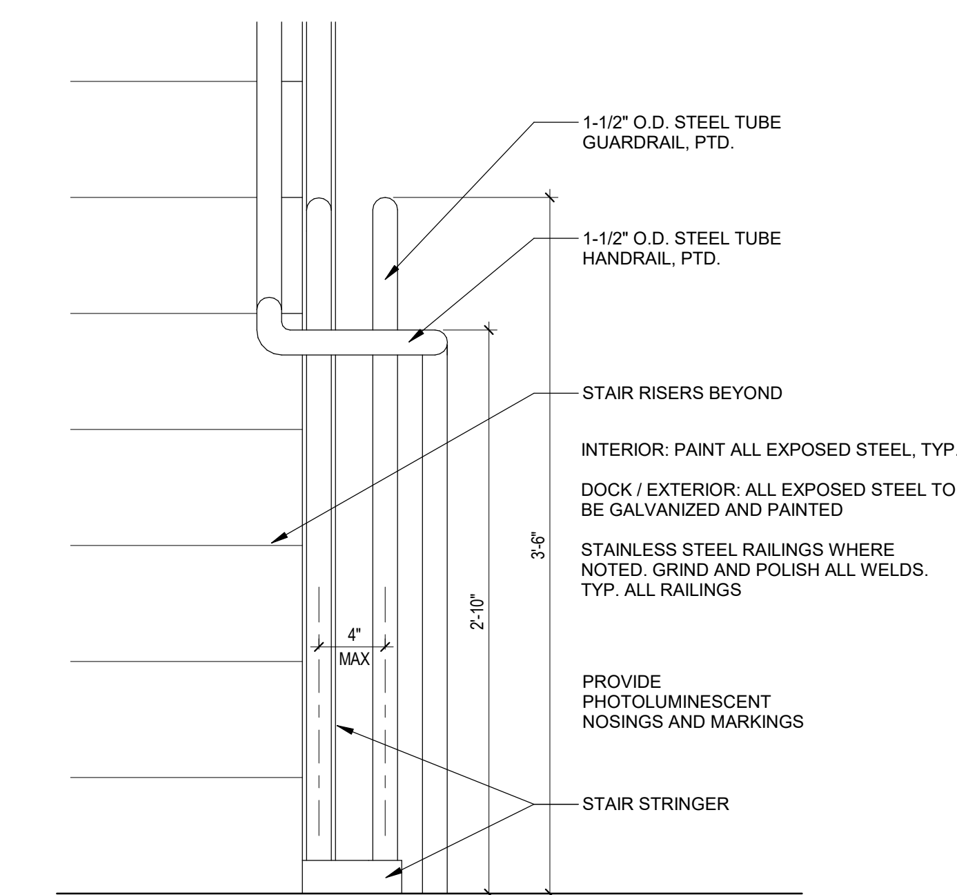
7 STAIR DETAIL - GUARDRAIL / HANDRAIL - ELEV AT LANDING 1 1/2" = 1'-0"
