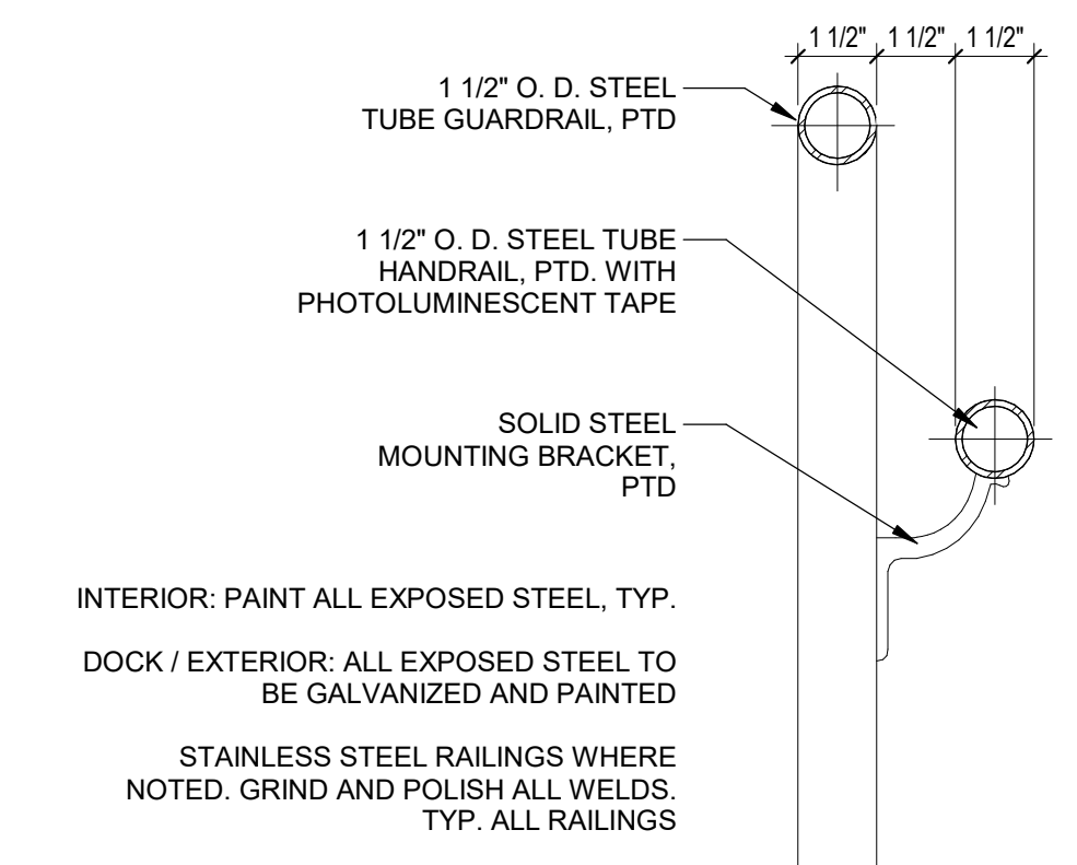
8 STAIR DETAIL - GUARDRAIL / HANDRAIL - SECTION - TYP 3" = 1'-0"
