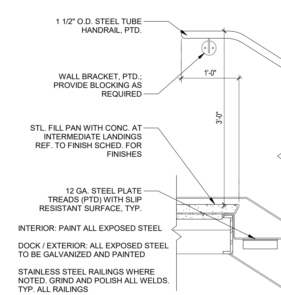
3 HANDRAIL ELEV. - WALL MOUNT - TOP OF STAIRS 1" = 1'-0"
