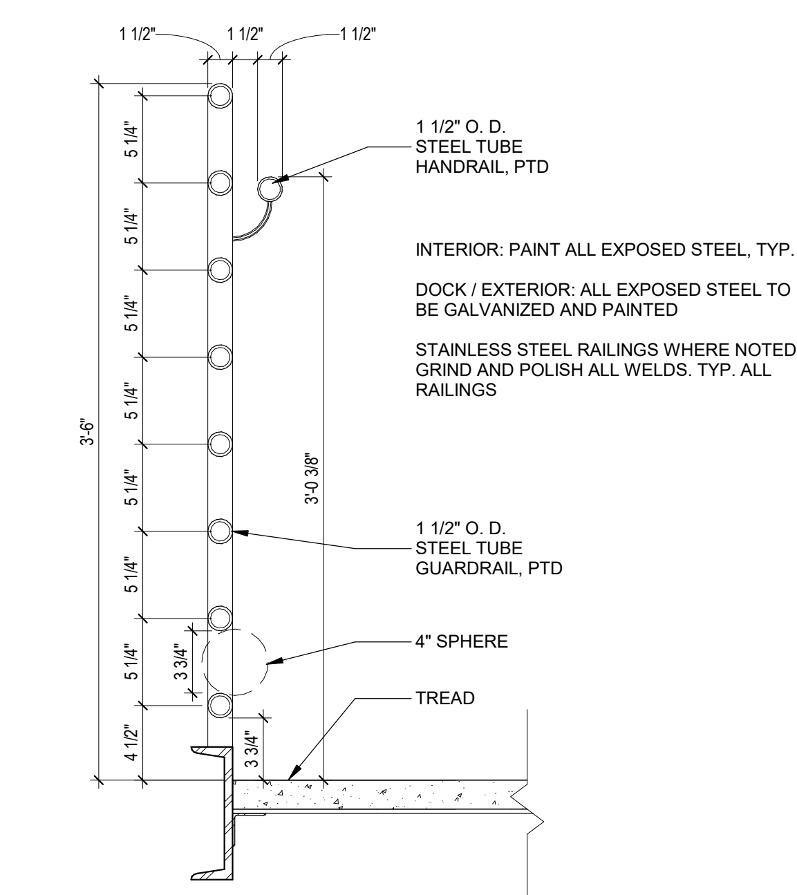
6 STAIR DETAIL - GUARDRAIL / HANDRAIL 1 1/2" = 1'-0"
