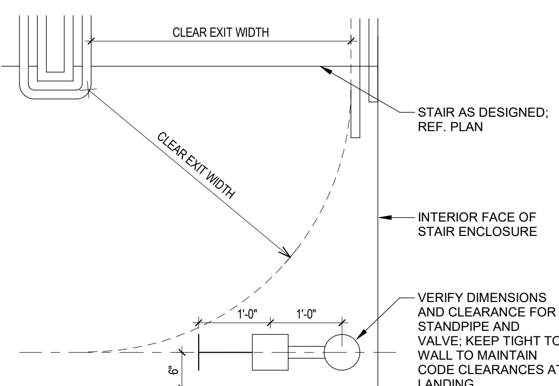
10 STAIR DETAIL - STANDPIPE CLEARANCE 3/4" = 1'-0"
