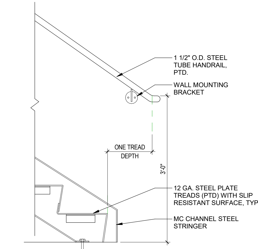
2 HANDRAIL ELEV. - WALL MOUNT - BOTTOM OF STAIRS 1" = 1'-0"
