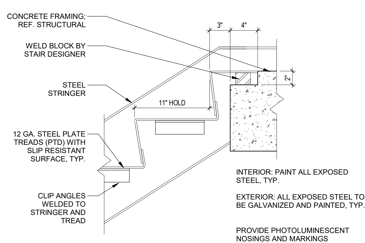
5 STAIR DETAIL - TREAD AND RISER @ TOP OF STAIR 1 1/2" = 1'-0"
