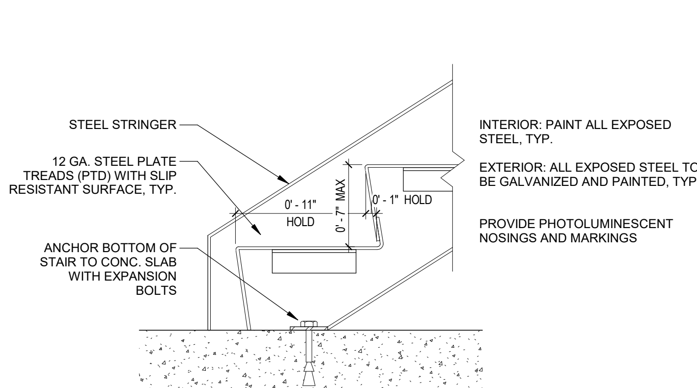
4 STAIR DETAIL - TREAD AND RISER - SECTION - AT BASE 1 1/2" = 1'-0"
