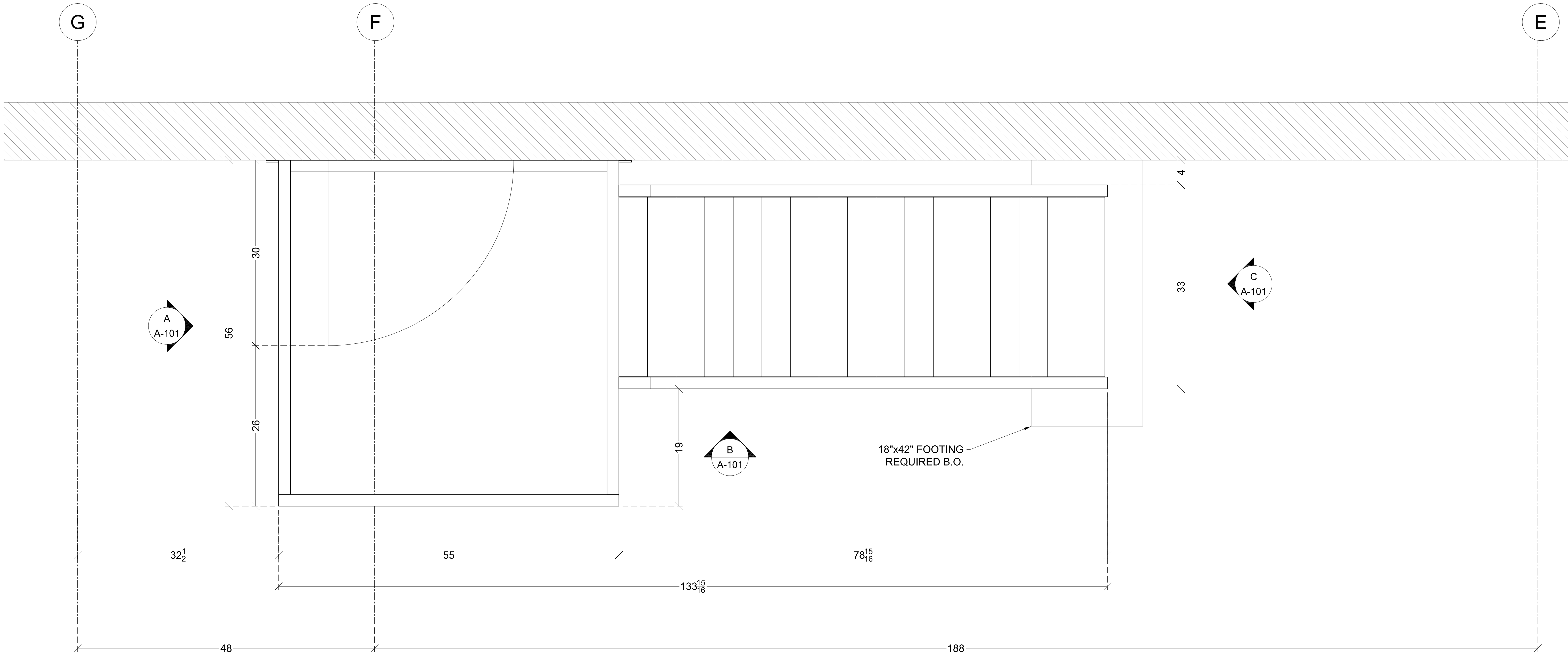
A SHIP LADDER - LAYOUT 1.5" = 12"
