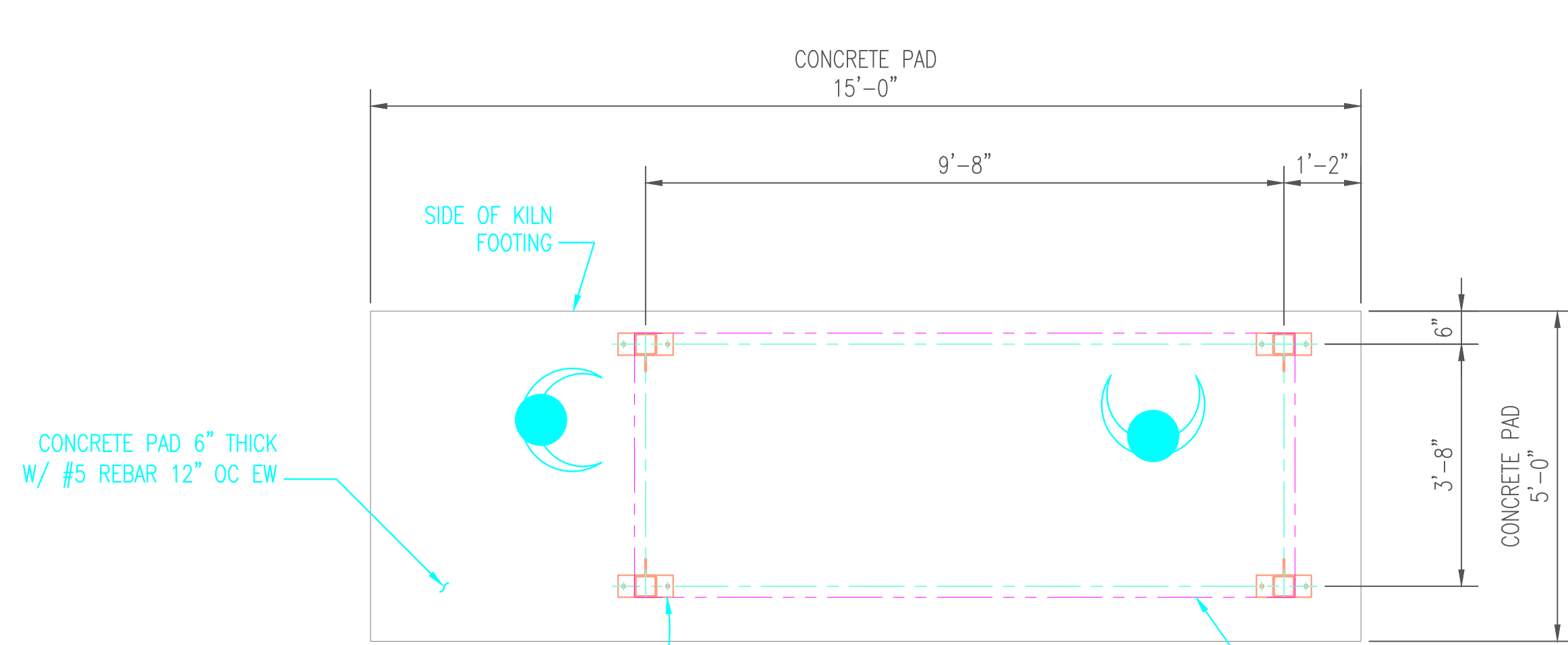
LAYOUT- PLAN
