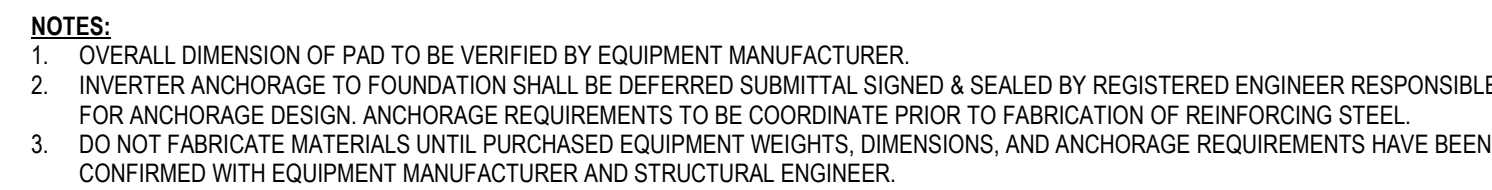
SECTION THRU INVERTER PAD OVERALL 1 SCALE: NO SCALE SE3-01
