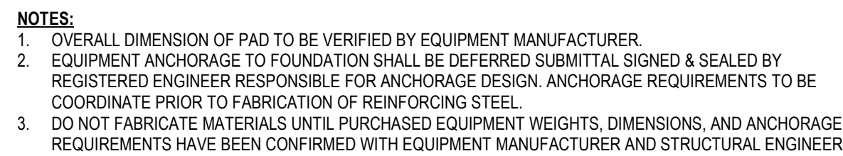
SECTION THRU EQUIPMENT PAD 9 SCALE: NO SCALE SE3-01
