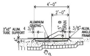
CROSS SECTION A SCALE: 3/8"=1'-0"
