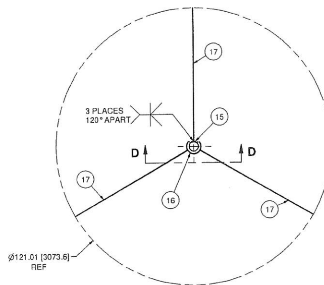
DETAIL: PIPE GUIDE ASSEMBLY
