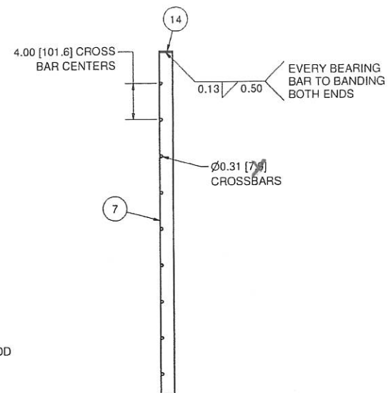
SECTION C-C
