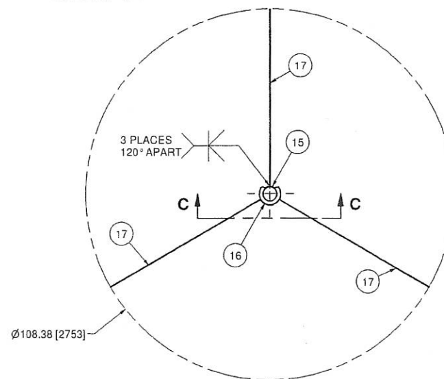
DETAIL: PIPE GUIDE ASSEMBLY
