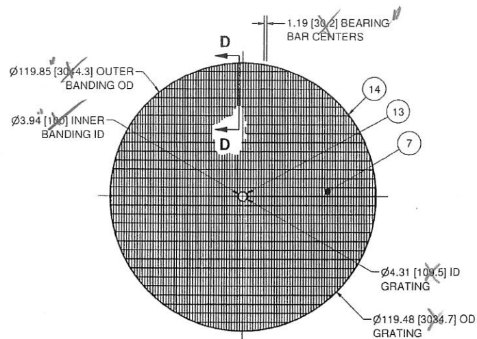
DETAIL: GRATING ASSEMBLY
