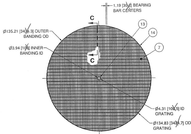
DETAIL: GRATING ASSEMBLY
